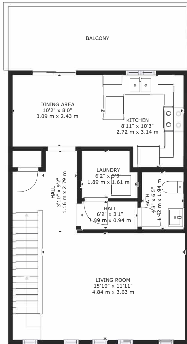
FLOOR 3 MAIN LEVEL
