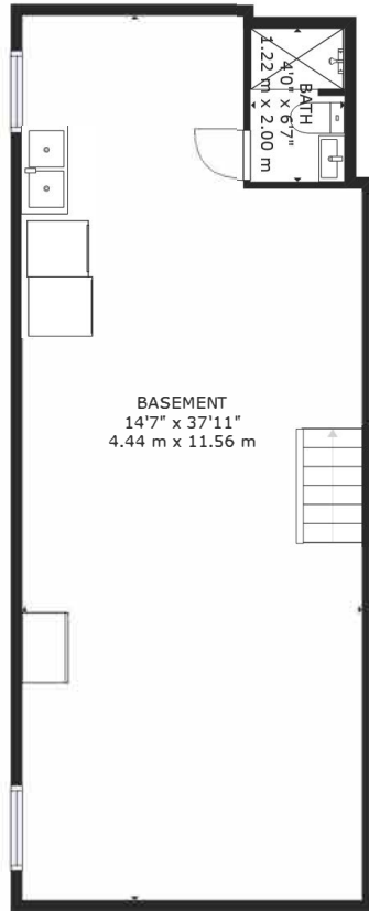
FLOOR 1 - LOWER LEVEL
