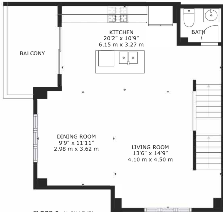
FLOOR 2 - MAIN LEVEL
