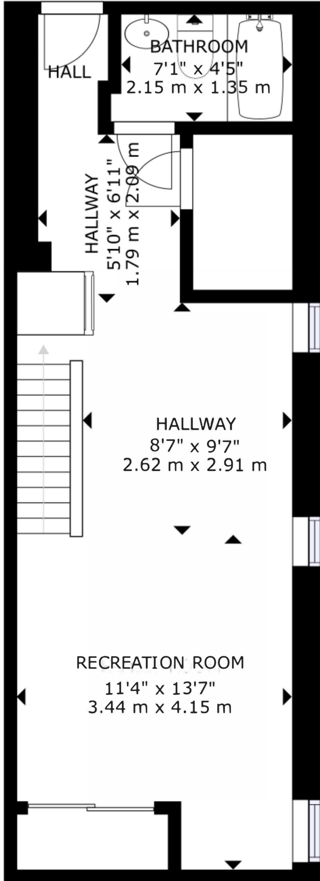
FLOOR 1 LOWER LEVEL
